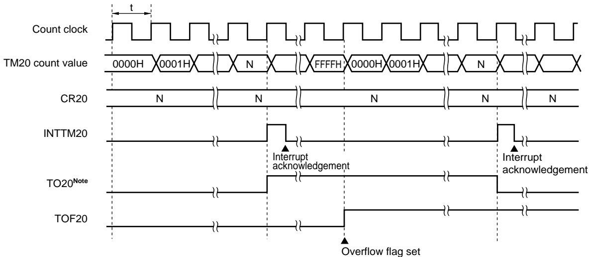
Figure 6-7. Timer Output Timing
